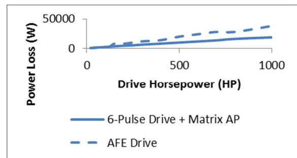
Figure 8 Power loss comparisons
