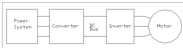
Figure 1 Basic VFD block diagram
