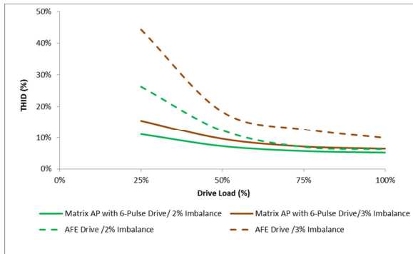
Figure 13 THID with system voltage imbalance comparison
