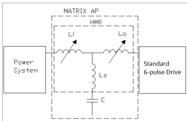
Figure 6 Matrix AP filter diagram
