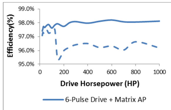
Figure 9 Efficiency Comparison
