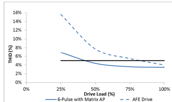
Figure 10 THID performance versus load comparison
