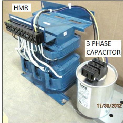
Figure 7 MTE MAPP0044D adaptive passive filter
