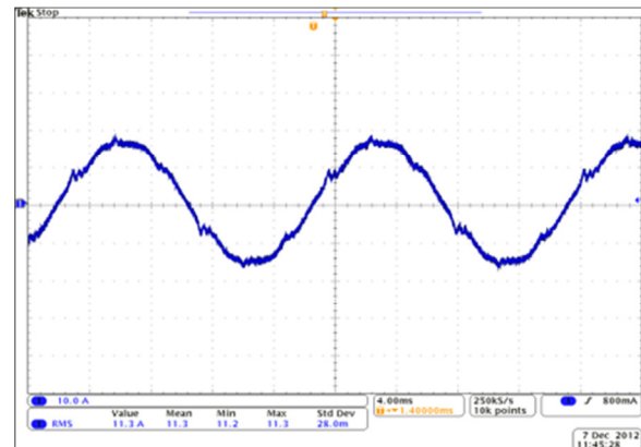
Figure 12 6-pulse drive with Matrix AP MAPP0044D input current waveform at 25% load
