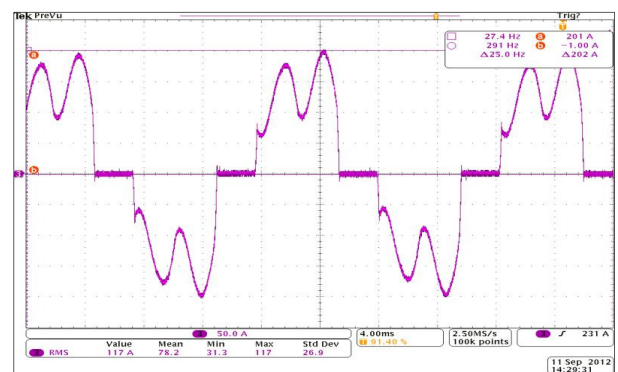
Figure 3 6-pulse unfiltered input current waveform
