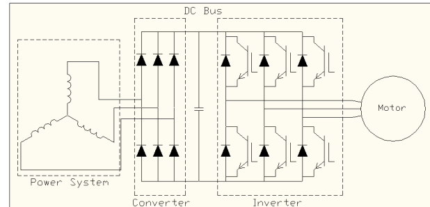
Figure 2 6-pulse power system and converter
