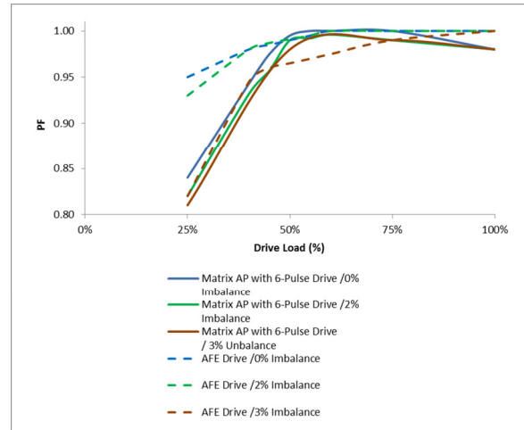
Figure 14 Power factor versus load comparison
