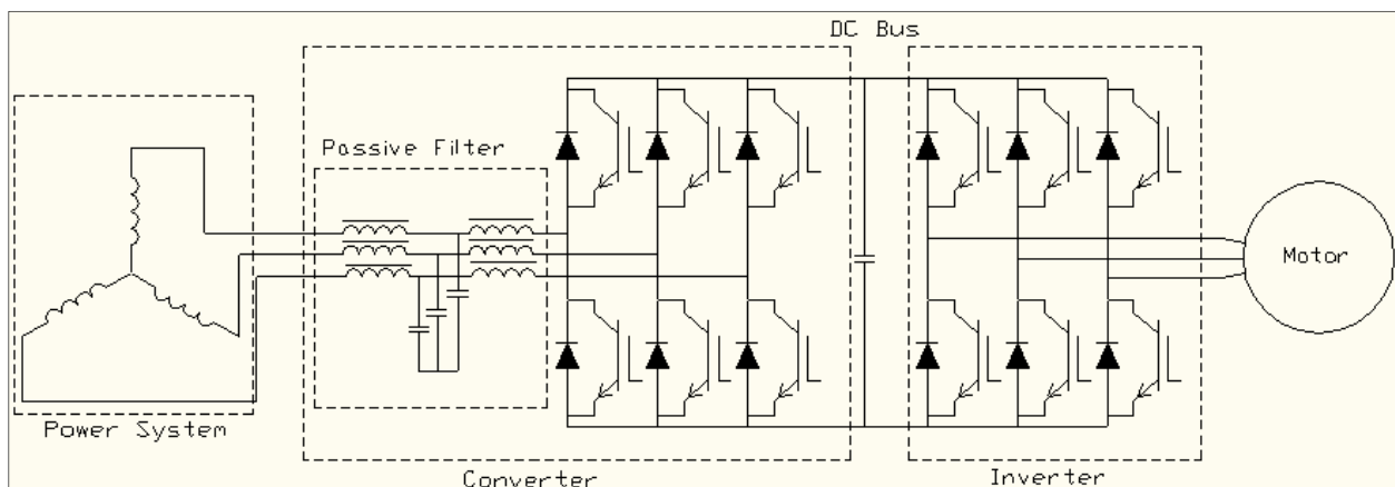
Figure 4 AFE Drive system
