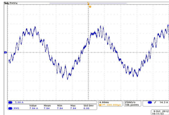
Figure 11 AFE input current waveform at 25% load
