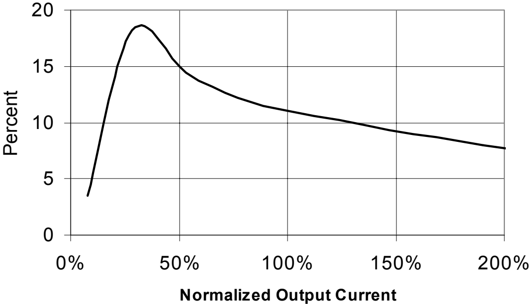
12% Filter w/DC Drive @ 250V Armature Nominal THID
