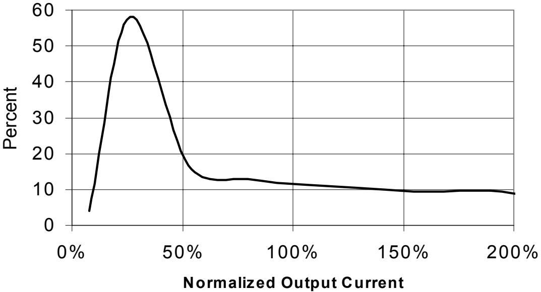
12% Filter w/DC Drive @ 50V Armature Nominal THID
