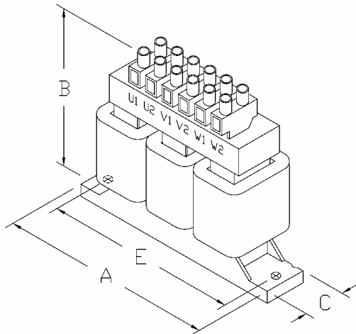
Figure 1 Snap Base Mount
